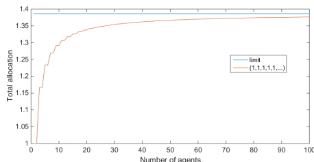
Figure 1: Optimal values of S for d = 1 . Figure 2: Optimal values of S for some 2-control vectors.
