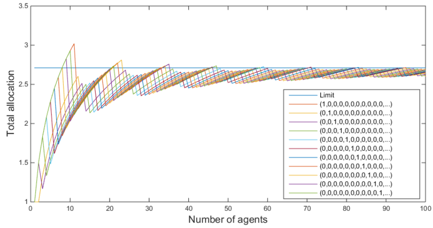
Figure 3: Optimal values of S for different control vectors when c = 10 .
