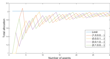
Figure 1: Optimal values of S for d = 1 . Figure 2: Optimal values of S for some 2-control vectors.
